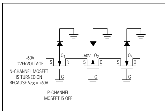
Figure 7. -60V Overvoltage with Multiplexer Power OFF
