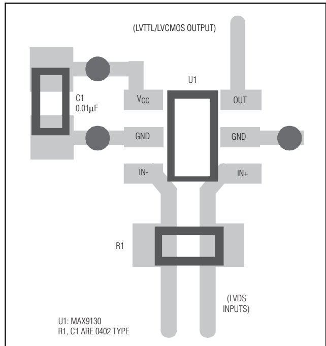
Figure 4. Board Layout
