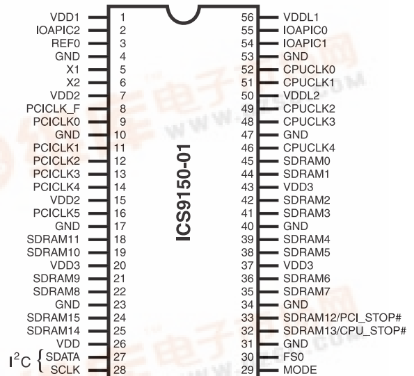
56-Pin SSOP
