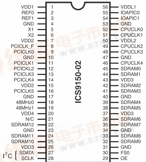
56-Pin SSOP
