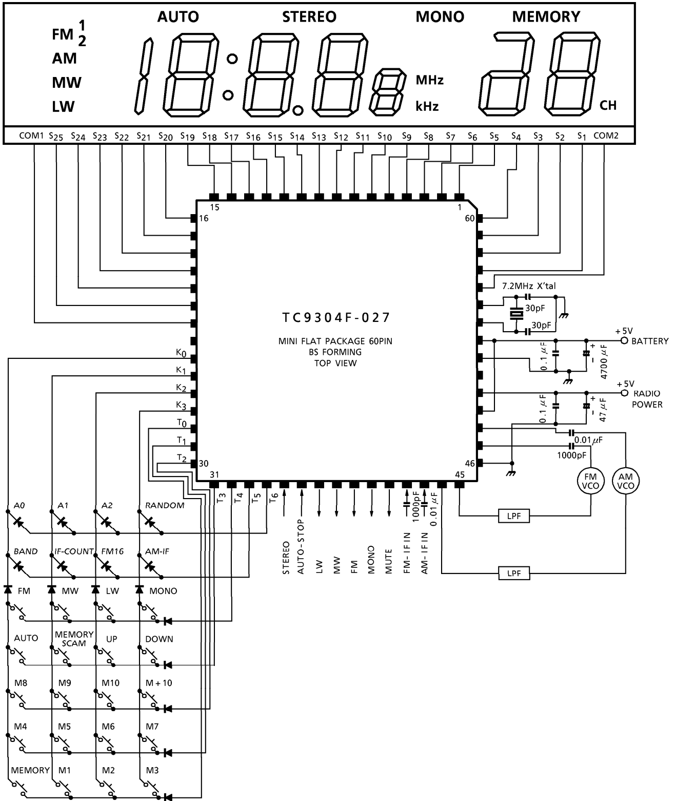
TC9304F-027 Layout
