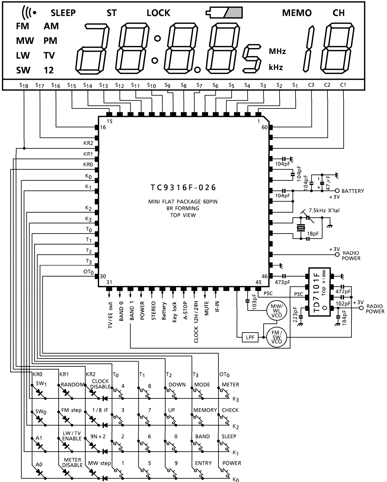
TC9316F-026 Layout
