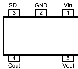
20041202 SOT23 - 5 Package (MF) Top View See NS package number MF05A
