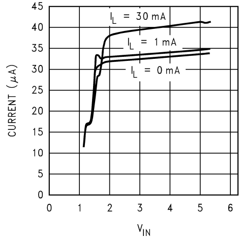
Ground Current vs V_{IN} at 125^\circ C
