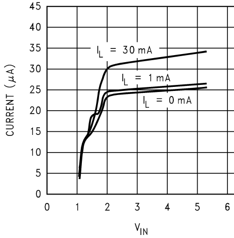
Ground Current vs V_{IN} at 25^\circ C
