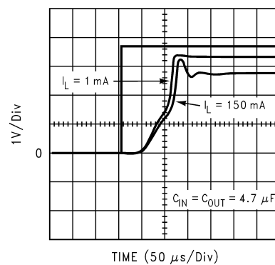
Enable Response
