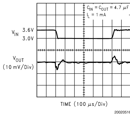
Line Transient Response (LP3988-2.85)
