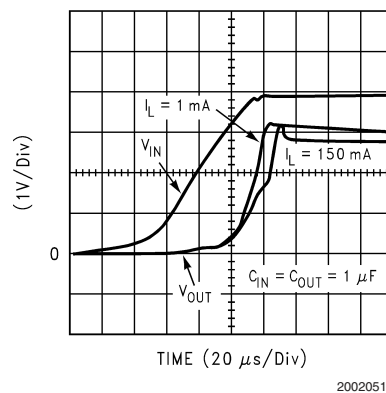
Power-Up Response
