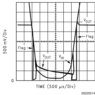
Line Transient Response (LP3988-2.85)
