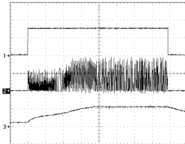
Start-Up/Shutdown
