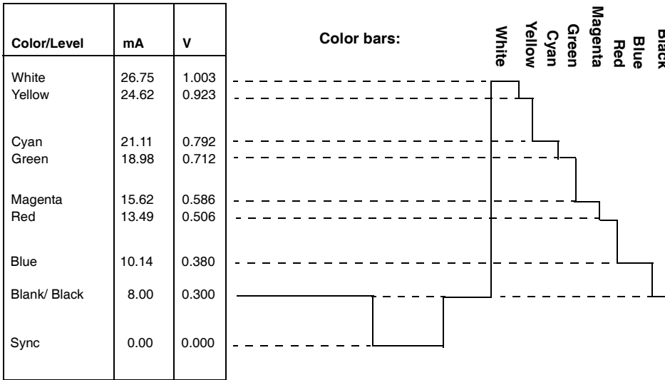
Figure 13: PAL Y (Luminance) Video Output Waveform (DACG = 1)
