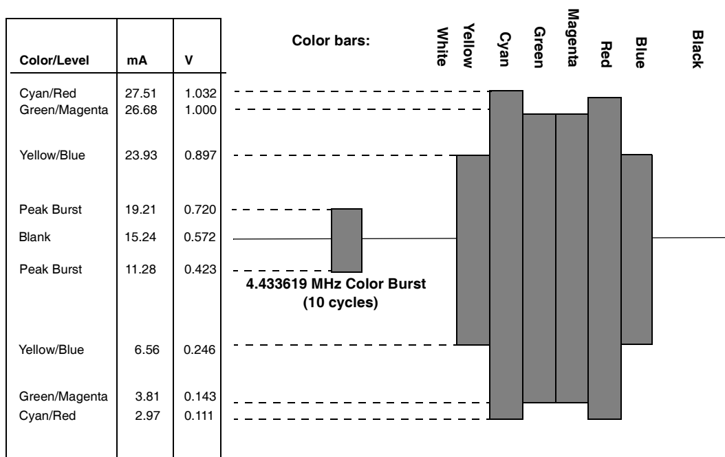
Figure 15: PAL C (Chrominance) Video Output Waveform (DACG = 1)
