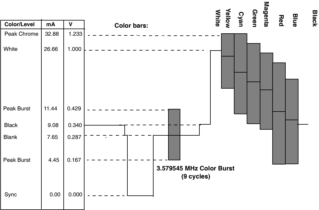
Figure 16: Composite NTSC Video Output Waveform (DACG = 0)
