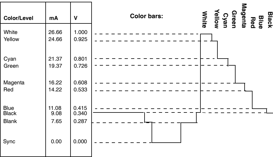
Figure 12: NTSC Y (Luminance) Output Waveform (DACG = 0)
