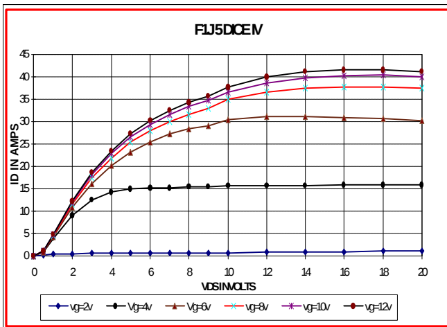
IV CURVE
