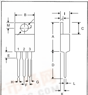
TO-220AB
