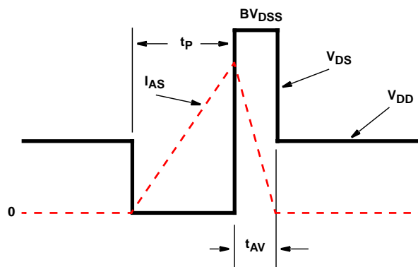
FIGURE 16. UNCLAMPED ENERGY WAVEFORM
