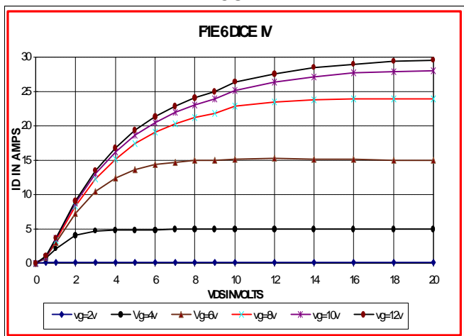
IV CURVE
