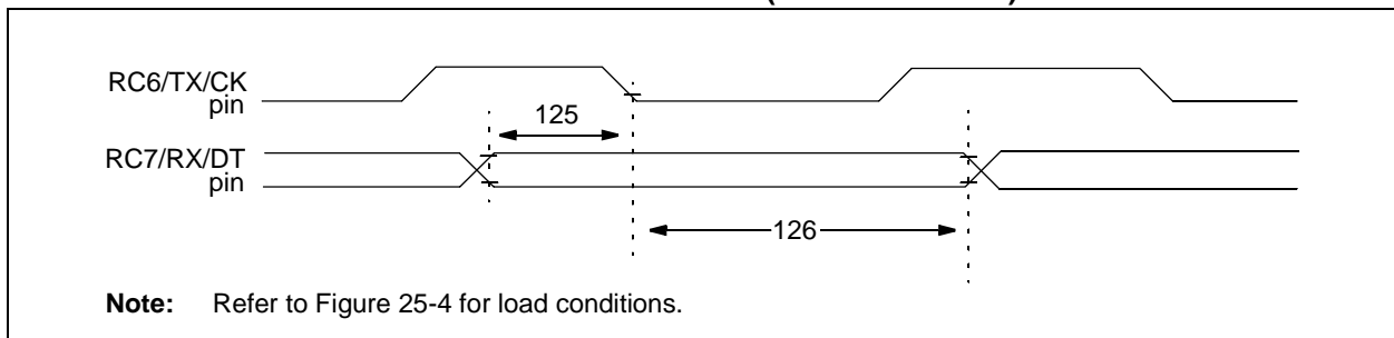
FIGURE 25-20: USART SYNCHRONOUS RECEIVE (MASTER/SLAVE) TIMING
