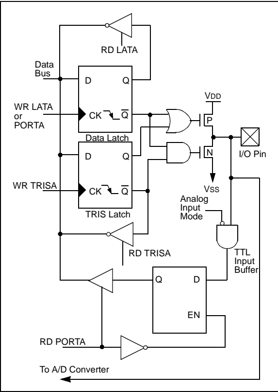
FIGURE 10-4: BLOCK DIAGRAM OF RA3:RA2 PINS
