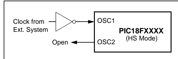
FIGURE 2-2: EXTERNAL CLOCK INPUT OPERATION (HS OSC CONFIGURATION)
