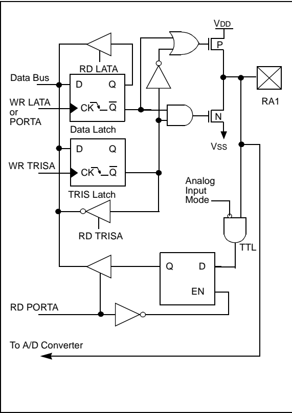
FIGURE 10-3: BLOCK DIAGRAM OF RA1
