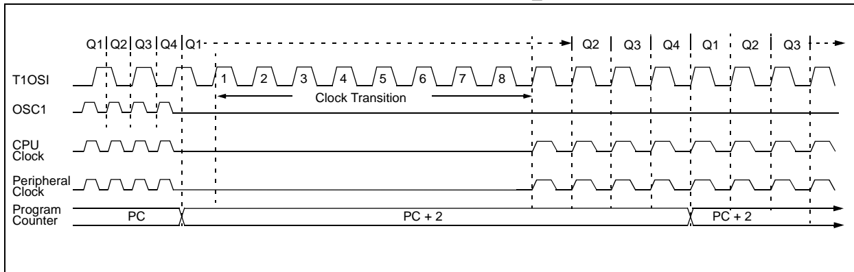
FIGURE 3-9: TIMING TRANSITION FOR ENTRY TO SEC_RUN MODE
