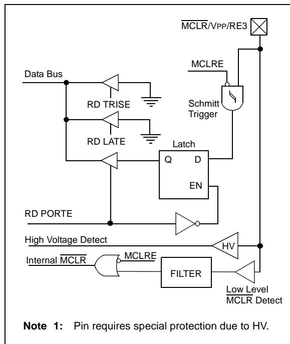
FIGURE 10-29: RE3 BLOCK DIAGRAM
