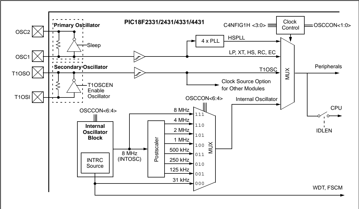
FIGURE 2-8: PIC18F2331/2431/4331/4431 CLOCK DIAGRAM
