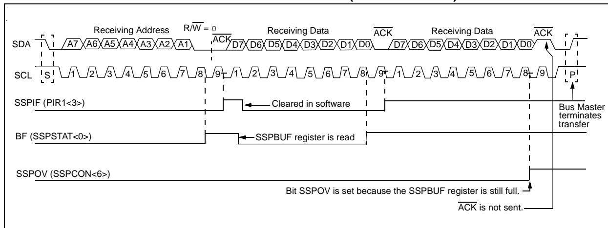
FIGURE 18-6: I 2 C WAVEFORMS FOR RECEPTION (7-BIT ADDRESS)
