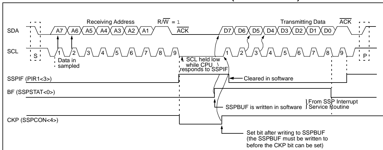
FIGURE 18-7: I 2 C WAVEFORMS FOR TRANSMISSION (7-BIT ADDRESS)
