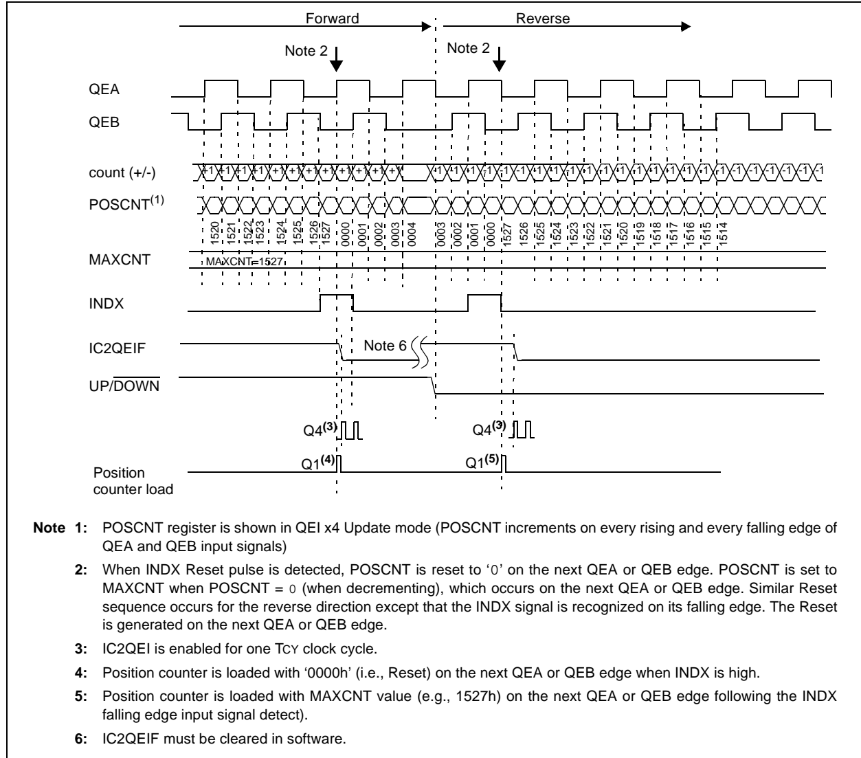
FIGURE 16-11: QE1 MODULE RESET TIMING WITH THE INDEX INPUT
