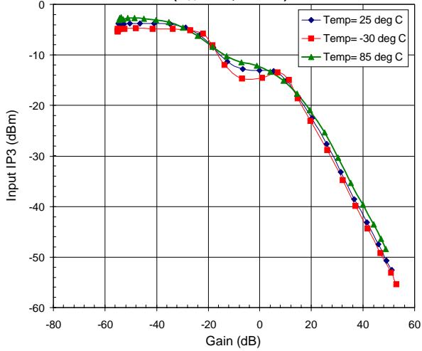
CDMA IIP3 versus Gain ( V_{CC}=3.0V , 85 MHz)
