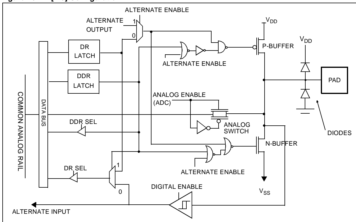
Figure 26. PA[7:0] Configuration
