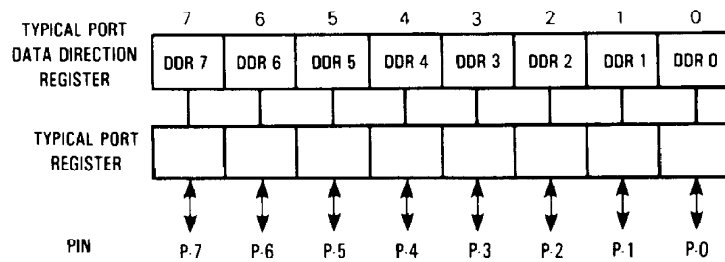
Figure 3. Typical Port I/O Circuitry and Register Configuration
