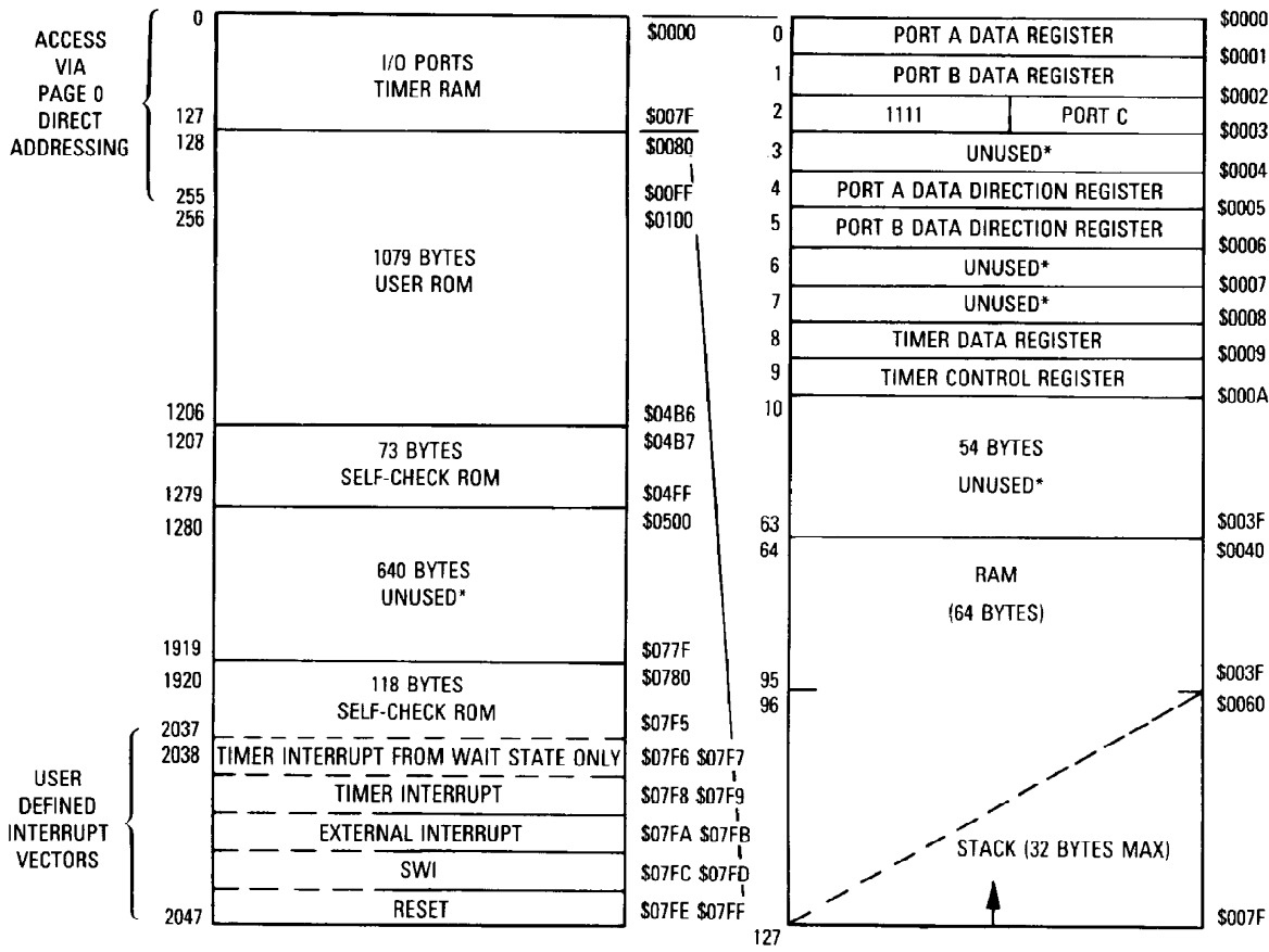
Figure 4. Memory Map
