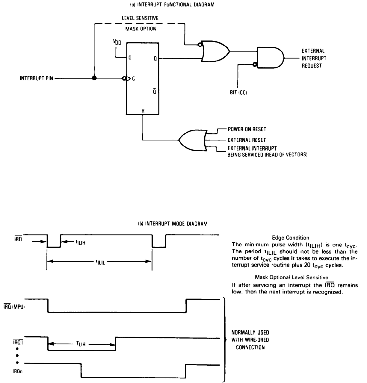
Figure 7. External Interrupt
