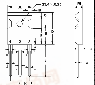
TO-247 (3P)
