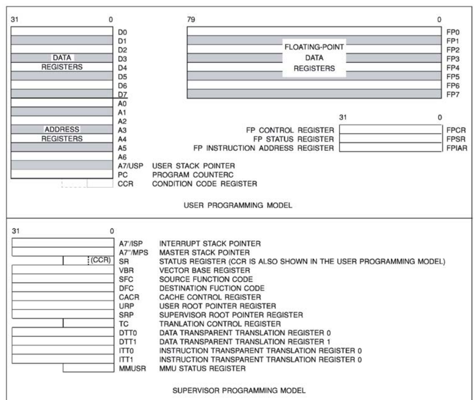
Figure 20. Programming Model
