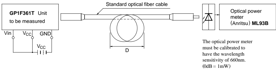
Fig. 1 Measuring Method Optical Output Coupling Fiber
