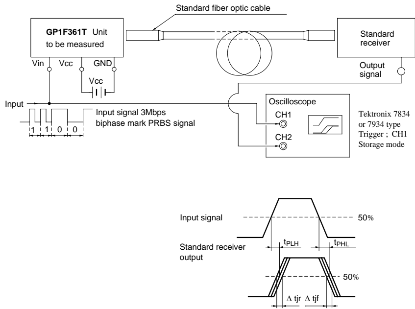
Fig. 3 Measuring Method of Pulse Response and Jitter
