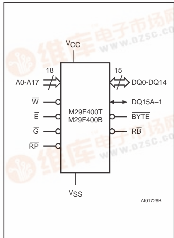
Figure 1. Logic Diagram
