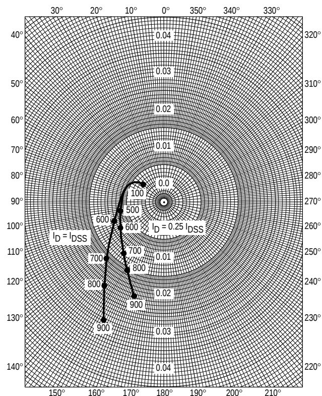
Figure 19. S12g
