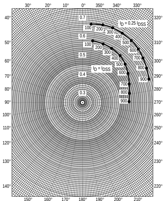
Figure 18. S11g
