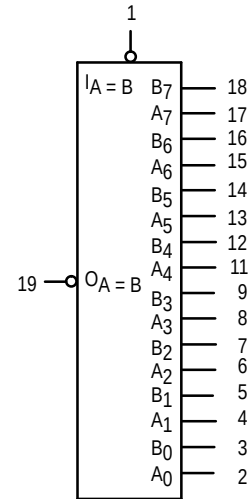
LOGIC SYMBOL
