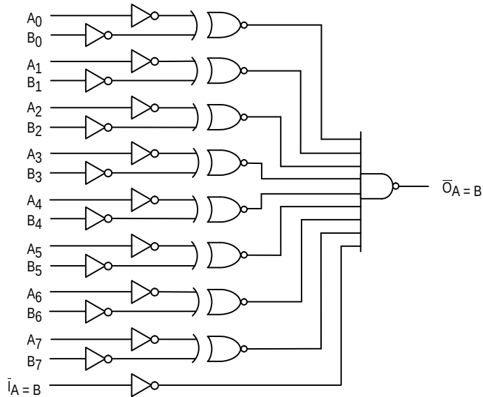
LOGIC DIAGRAM
