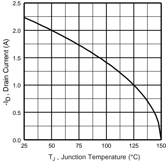
Fig 9. Maximum Drain Current Vs. Junction Temperature
