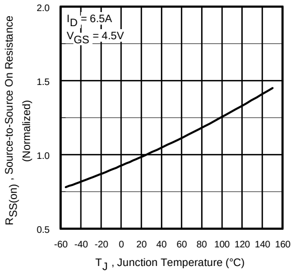
Fig 8. Normalized On-Resistance vs. Temperature. ⑤
