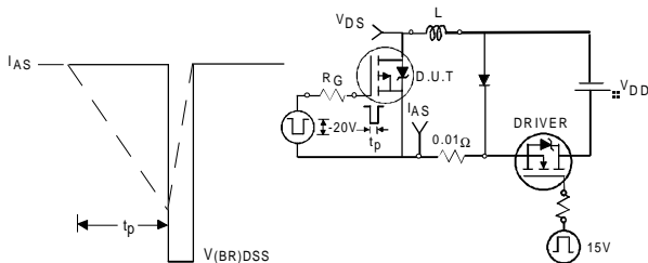
Fig 15a&b. Unclamped Inductive Test circuit and Waveforms
