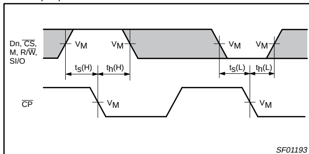
Waveform 2. Setup and Hold Times
