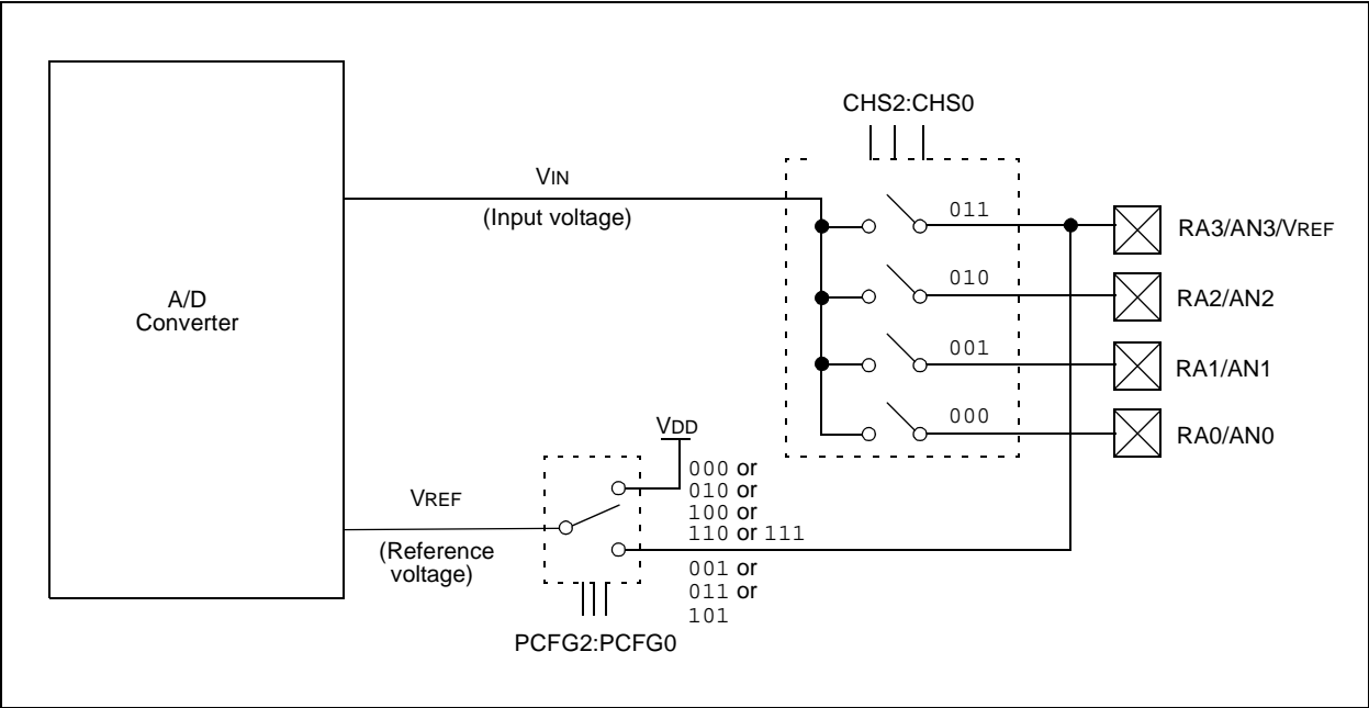
FIGURE 8-1: A/D BLOCK DIAGRAM
