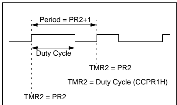
FIGURE 7-4: PWM OUTPUT
