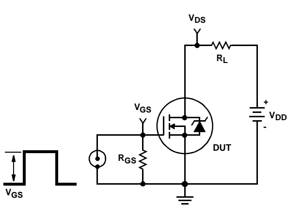
FIGURE 18. SWITCHING TIME TEST CIRCUIT
