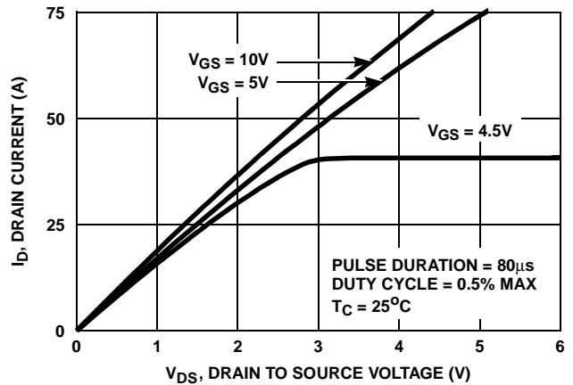
FIGURE 8. SATURATION CHARACTERISTICS
