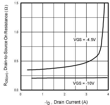
Fig 16. Typical On-Resistance Vs. Drain Current
