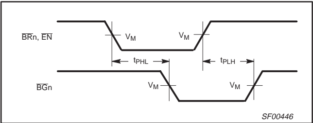
Waveform 2. Propagation delay for bus request or enable to bus grant output
