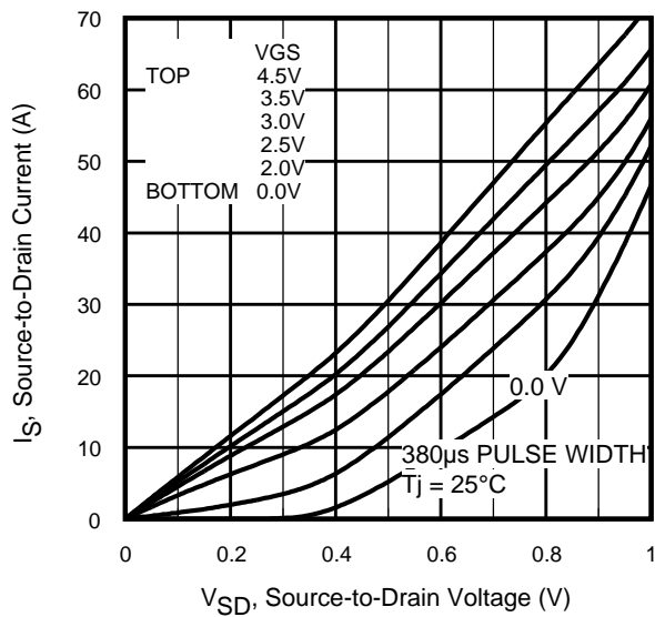
Fig 3. Typical Reverse Output Characteristics
