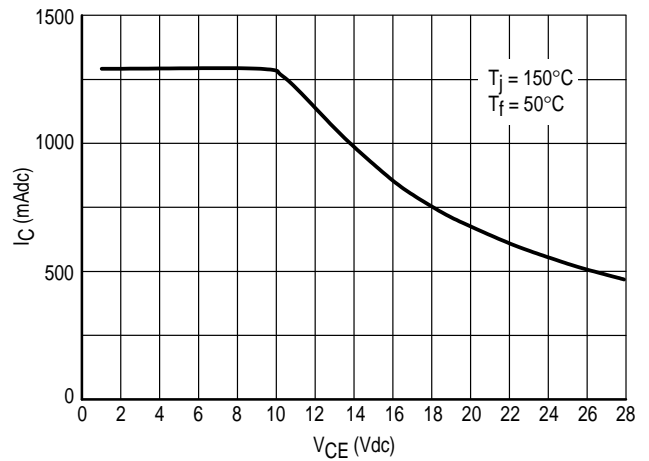
Figure 4. MRF857S DC SOA
