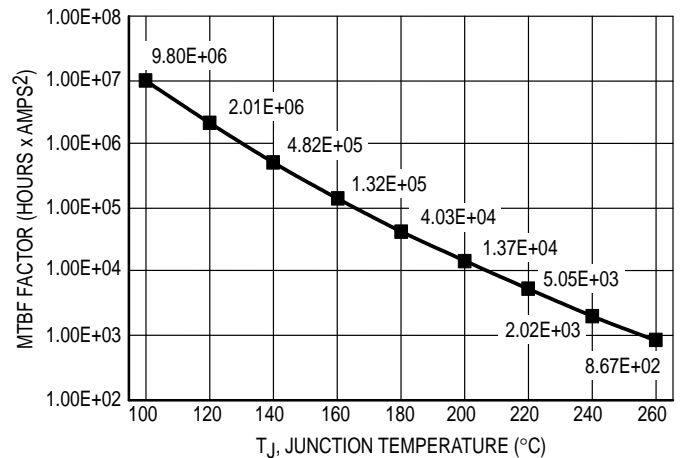
Figure 6. MRF857S MTBF Factor versus Junction Temperature
