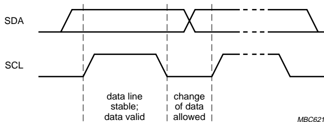
Fig.15 Bit transfer.
