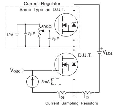
Fig 15. Gate Charge Test Circuit
