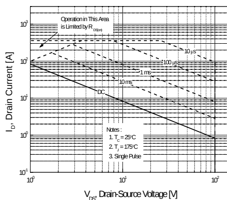
Figure 9-2. Maximum Safe Operating Area for FQPF90N10V2
