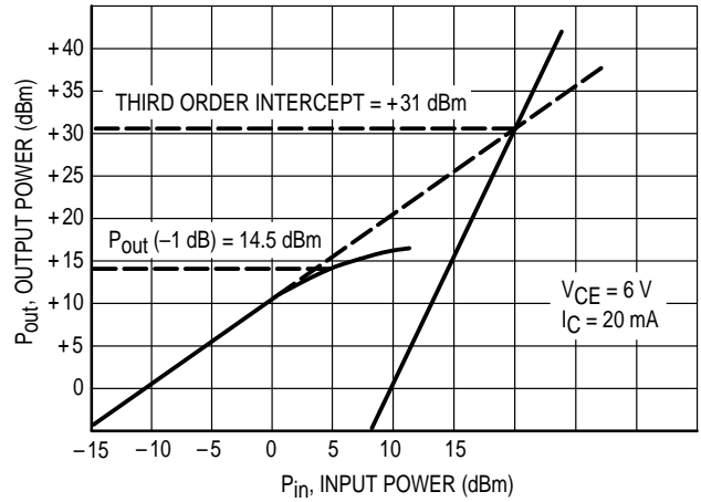
Figure 16. Third Order Intercept and 1 dB Compression Point
