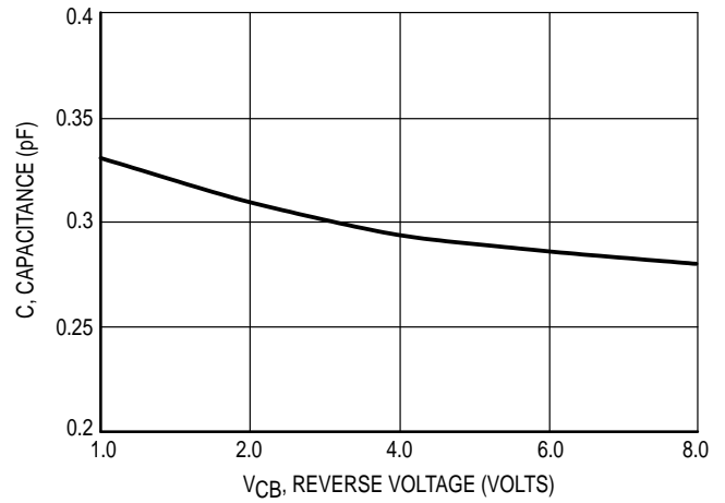
Figure 2. C_{iC} , Collector-Base Capacitance versus Voltage
