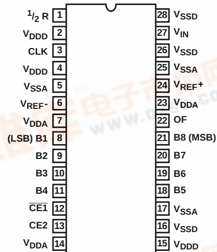
HS-900RH (FLATPACK) CDFP3-F28 TOP VIEW
