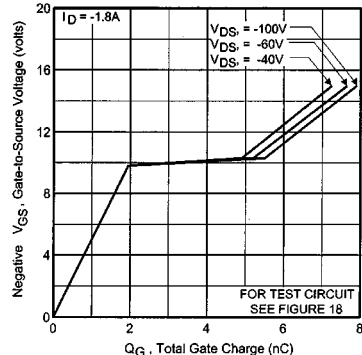
Fig. 11 — Typical Gate Charge Vs. Negative VGS - Gate-to-Source Voltage
