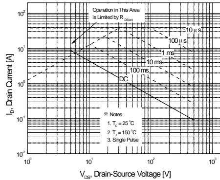
Figure 9-2. Maximum Safe Operating Area for FQP9N50C
