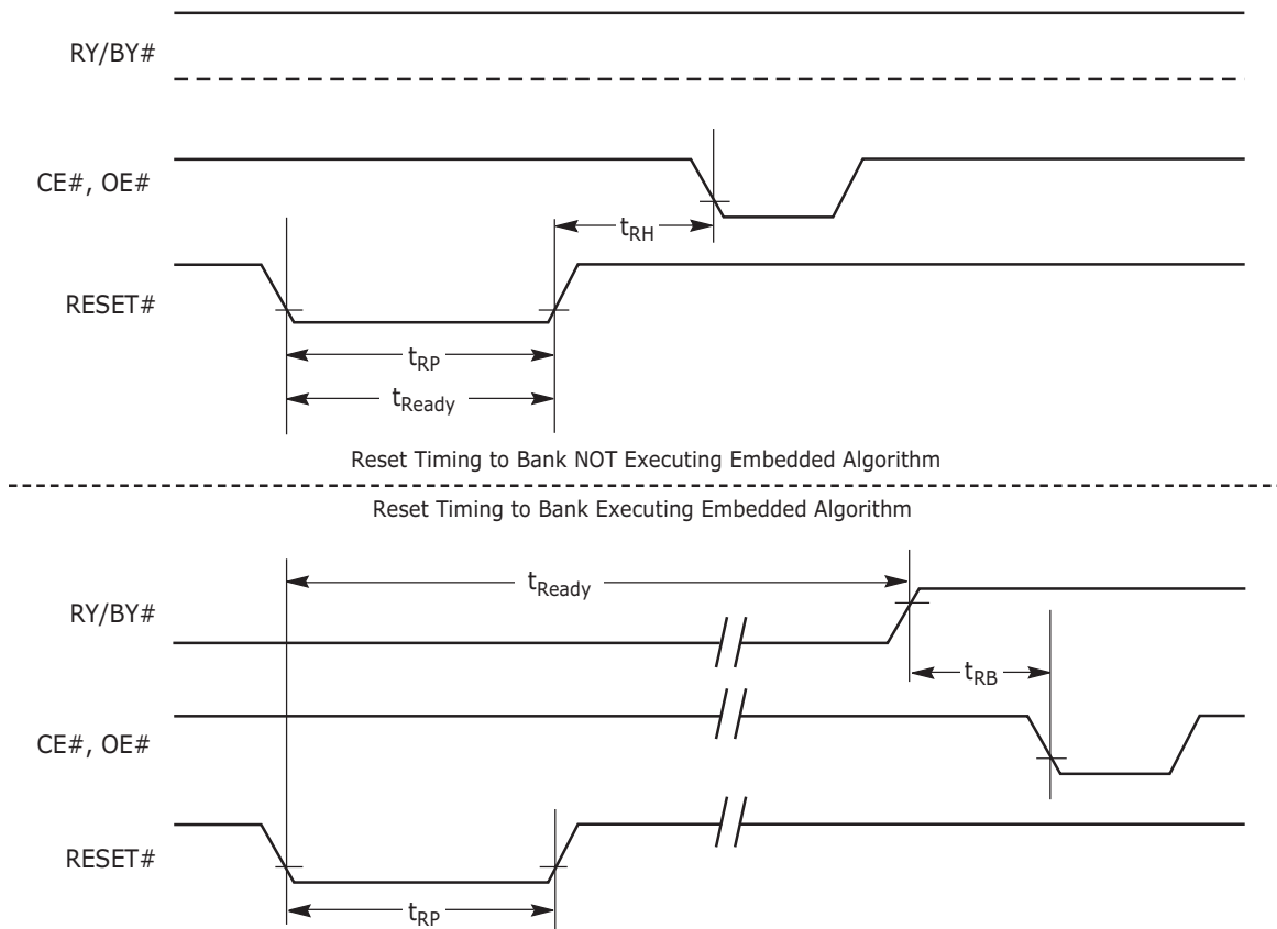
Figure I9. RESET# Timings
