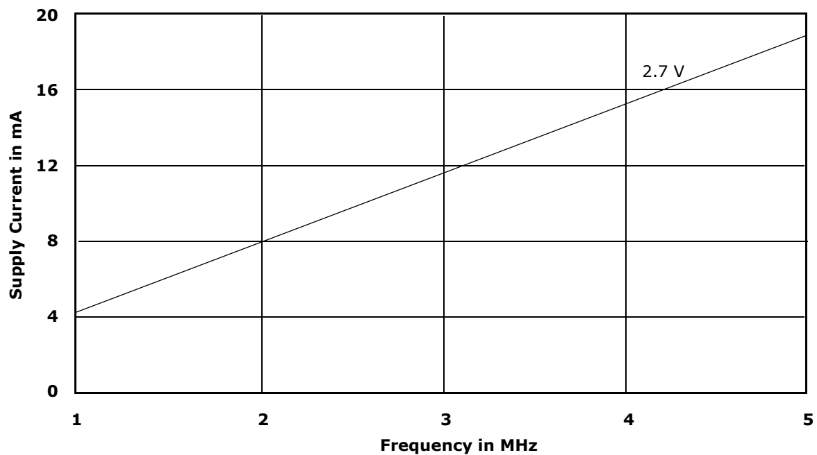
Figure 11. Typical I_{CCI} vs. Frequency
