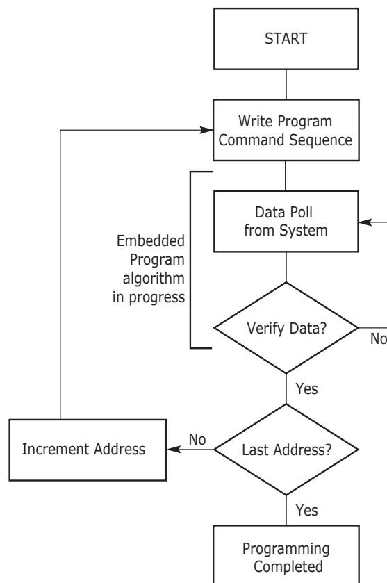
Figure 4. Program Operation
