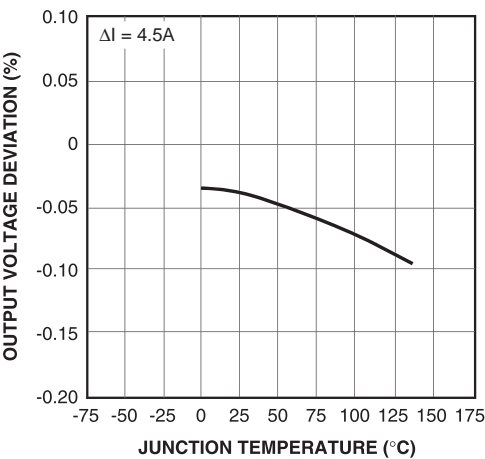
Figure 3. Load Regulation vs. Temperature
