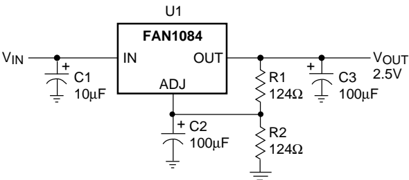
Figure 6. Application Circuit
