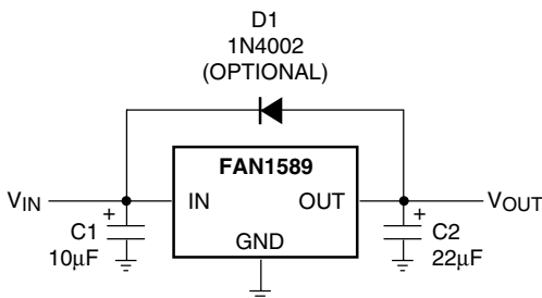
Figure 9. Optional Protection
