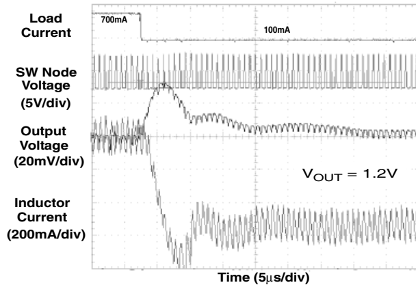
Transient Response
