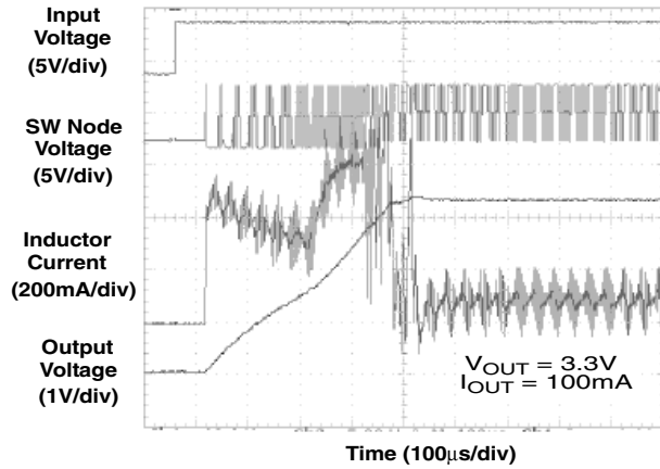
Start-up Response
