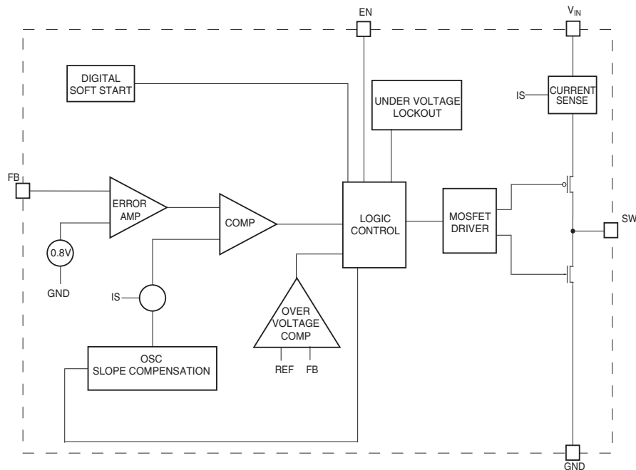
Figure 4. Block Diagram
