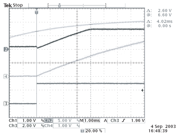
Figure 2. Start-Up Waveforms
