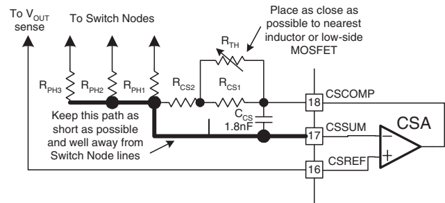
Figure 5. Temperature Compensation Circuit
