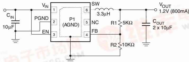
Figure 1. Typical Application
