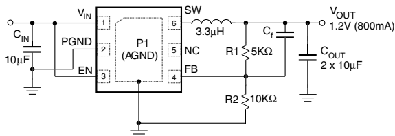
Figure 4. Setting the Output Voltage
