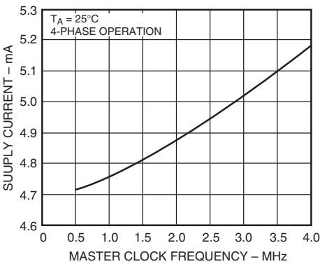
TPC 2. Supply Current vs. Master Clock Frequency
