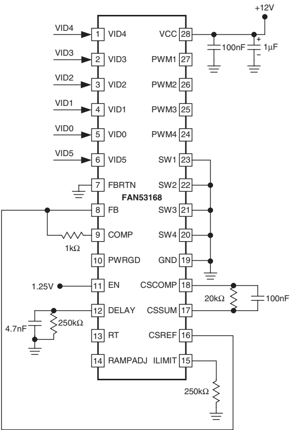
Test Circuit 3 – Closed Loop Output Voltage Accuracy
