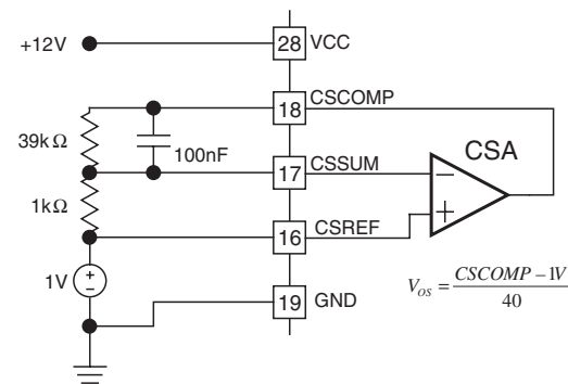
Test Circuit 1 – Current Sense Amplifier V_{os}
